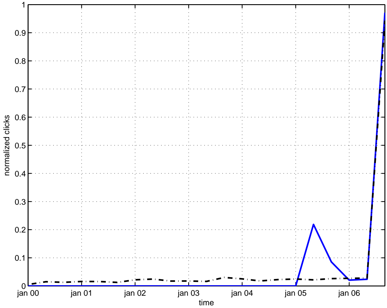
topological vertex
