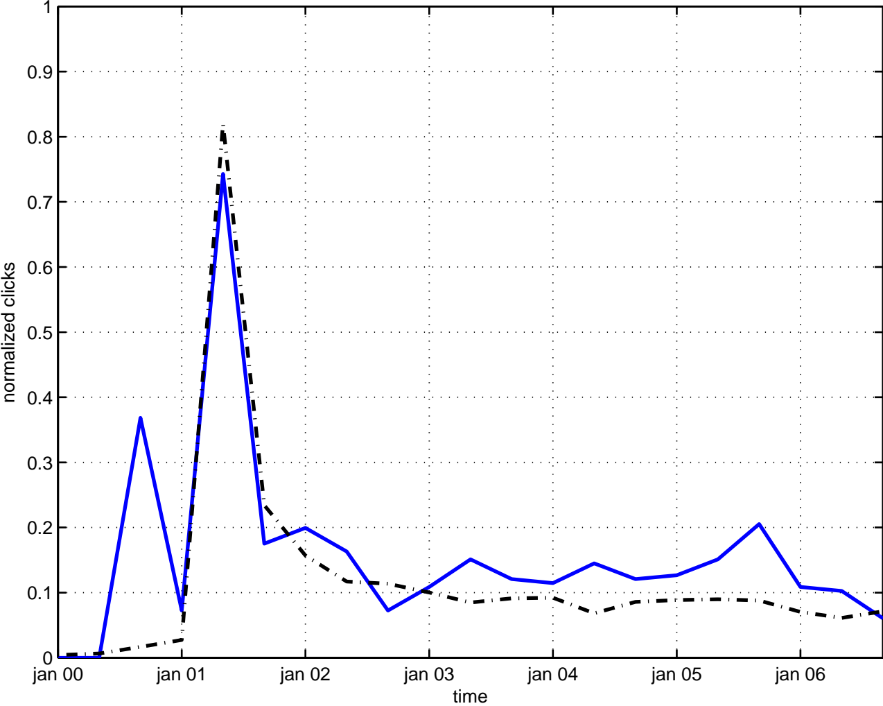
topological symmetry breaking
