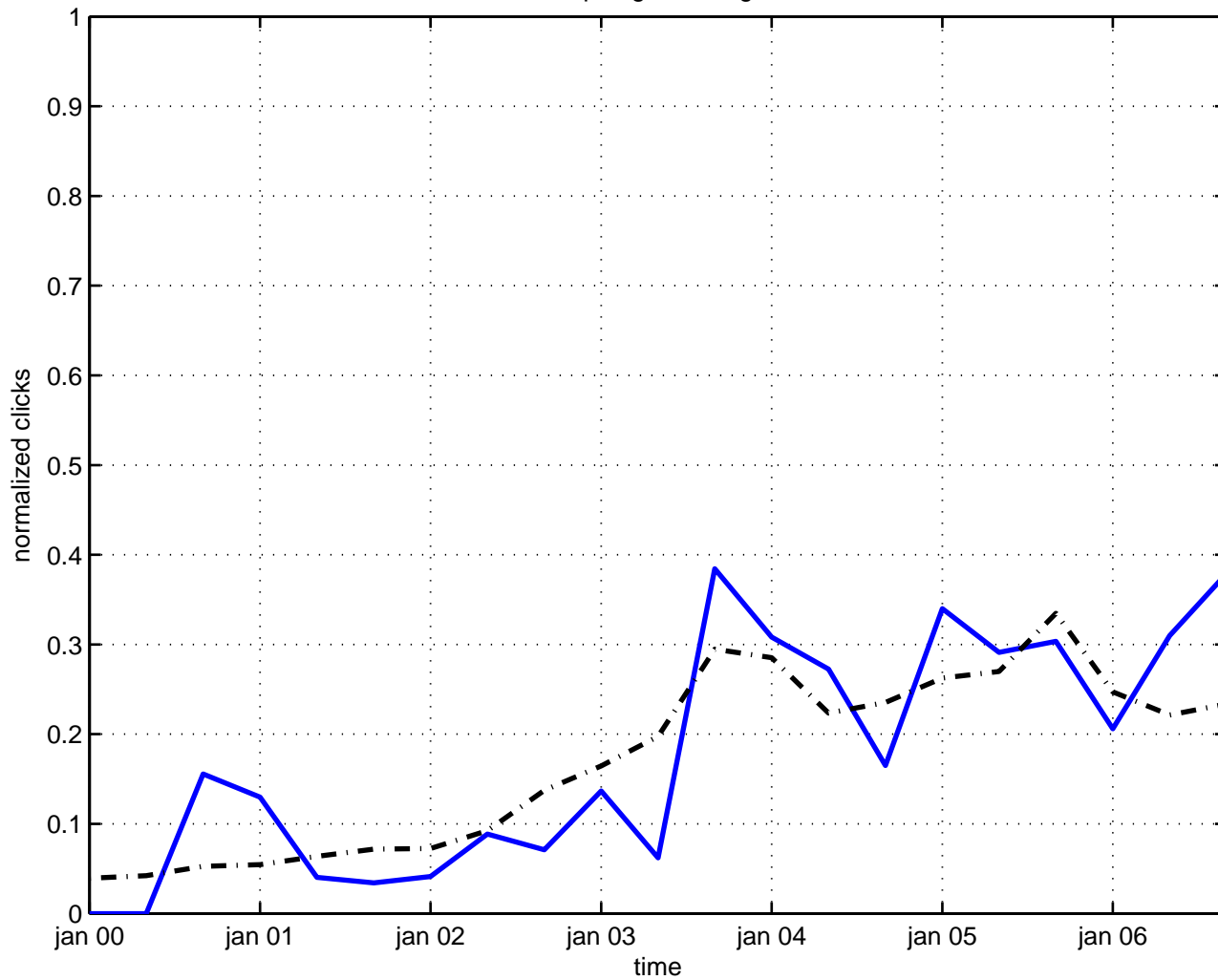
topological string
