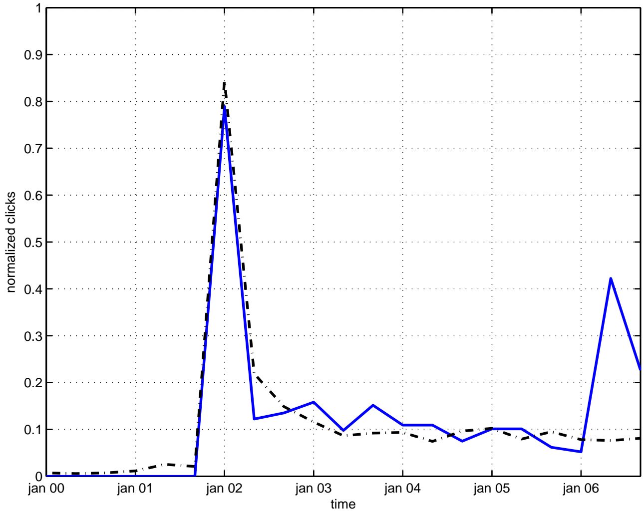
topological space
