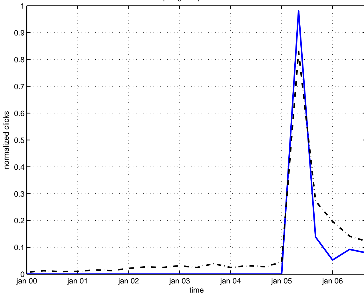
topological quantization
