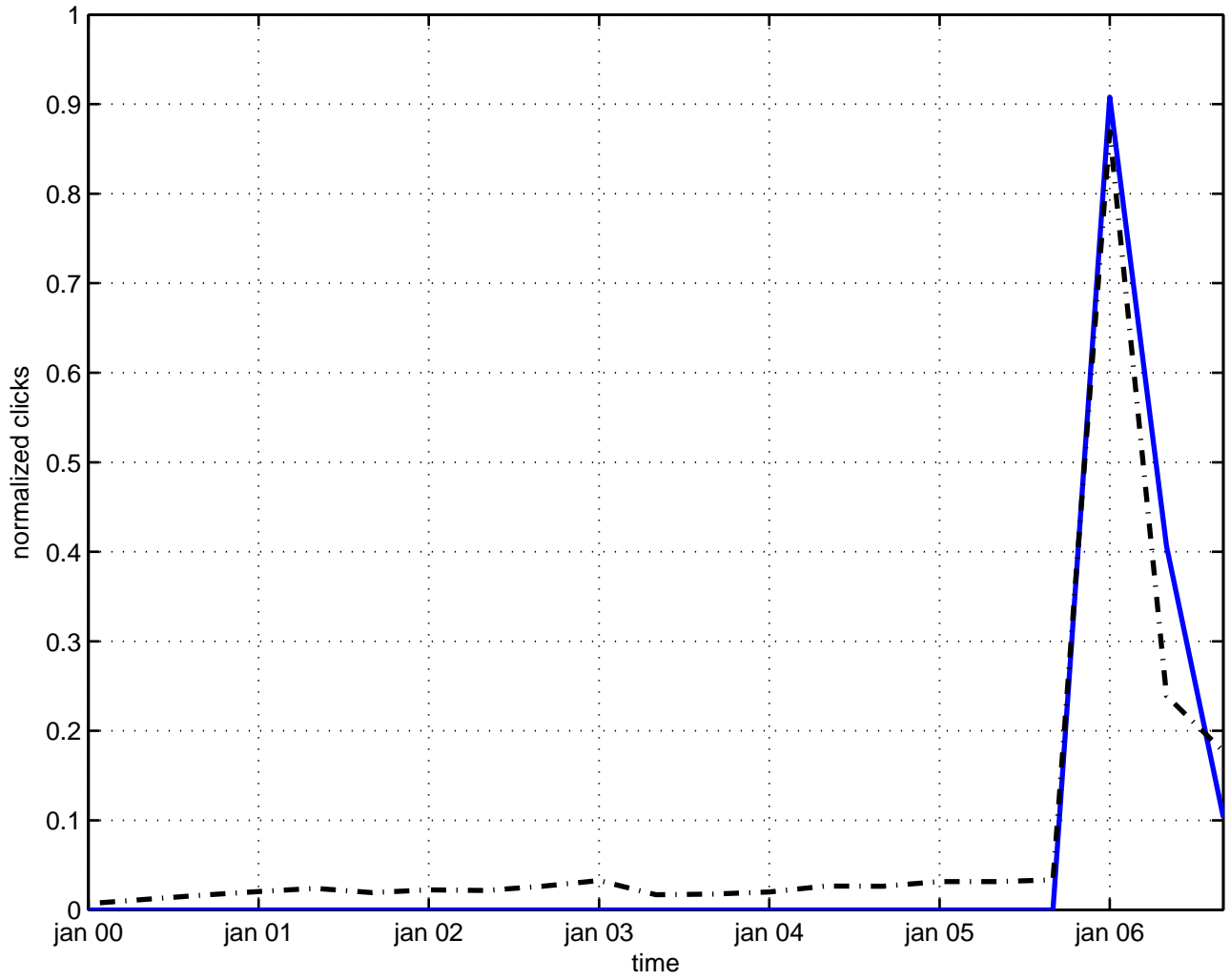
topological q-ball
