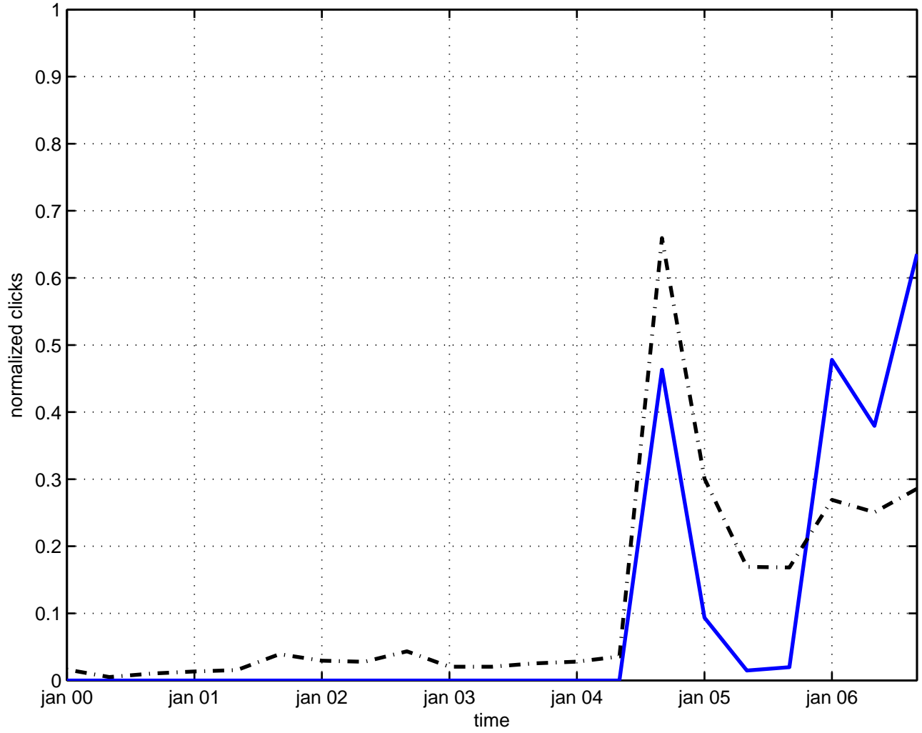
topological phase
