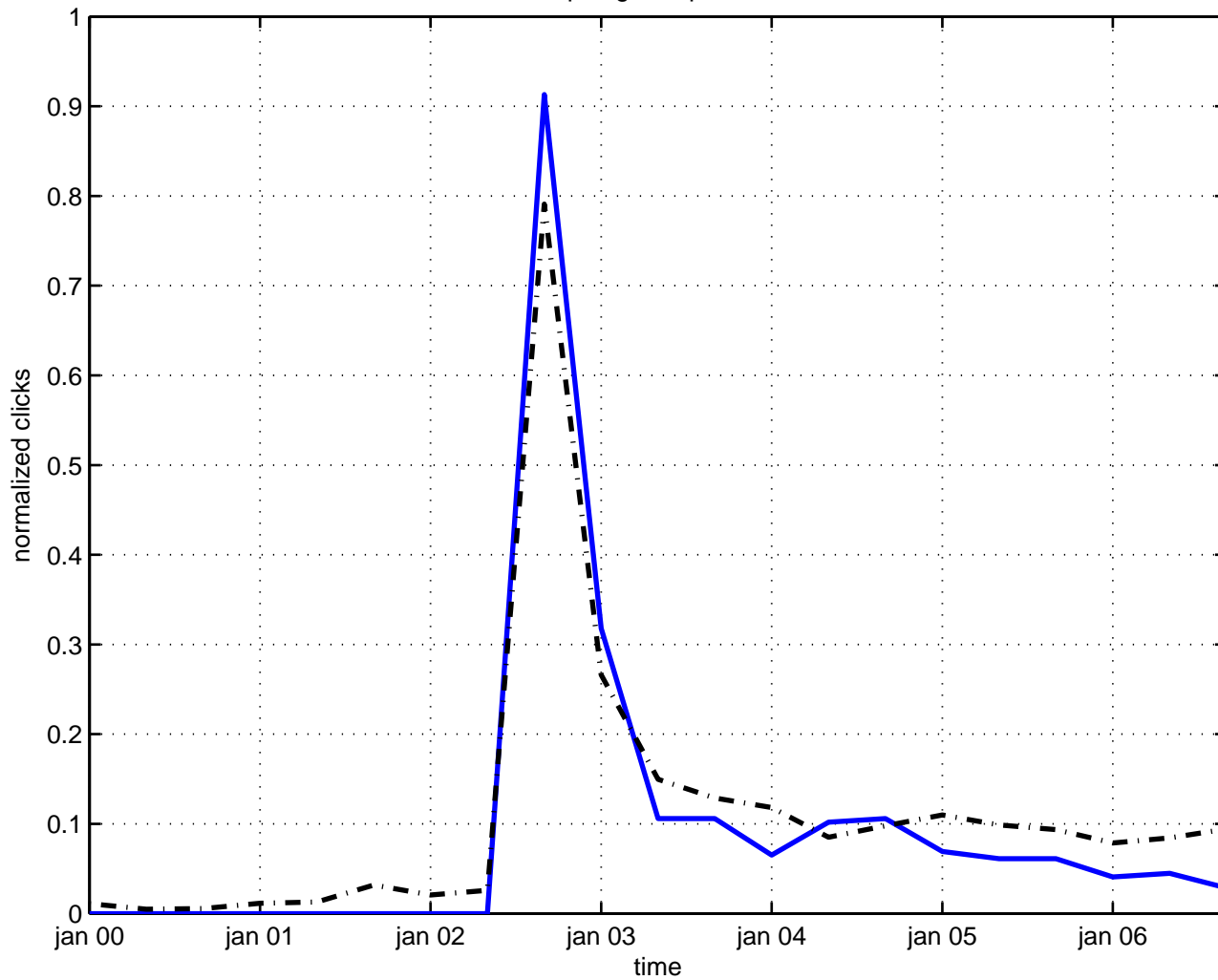
topological operator
