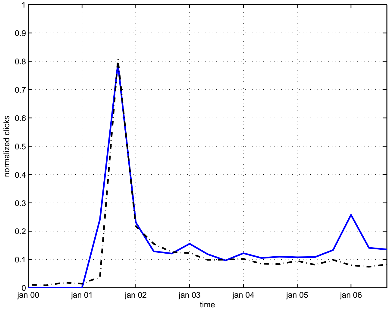
topological model
