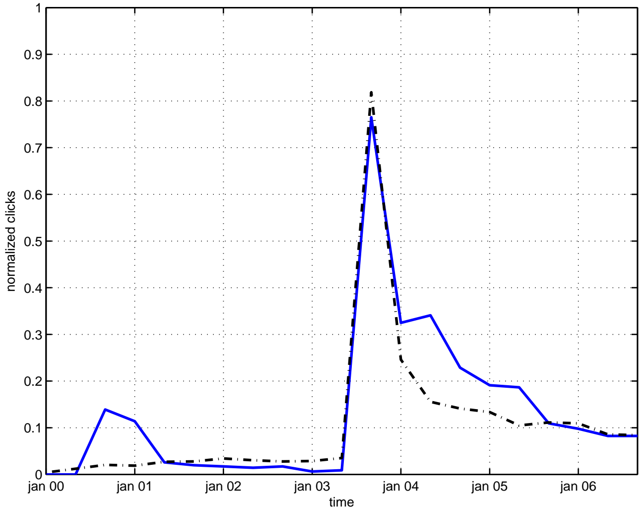
topological matrix model
