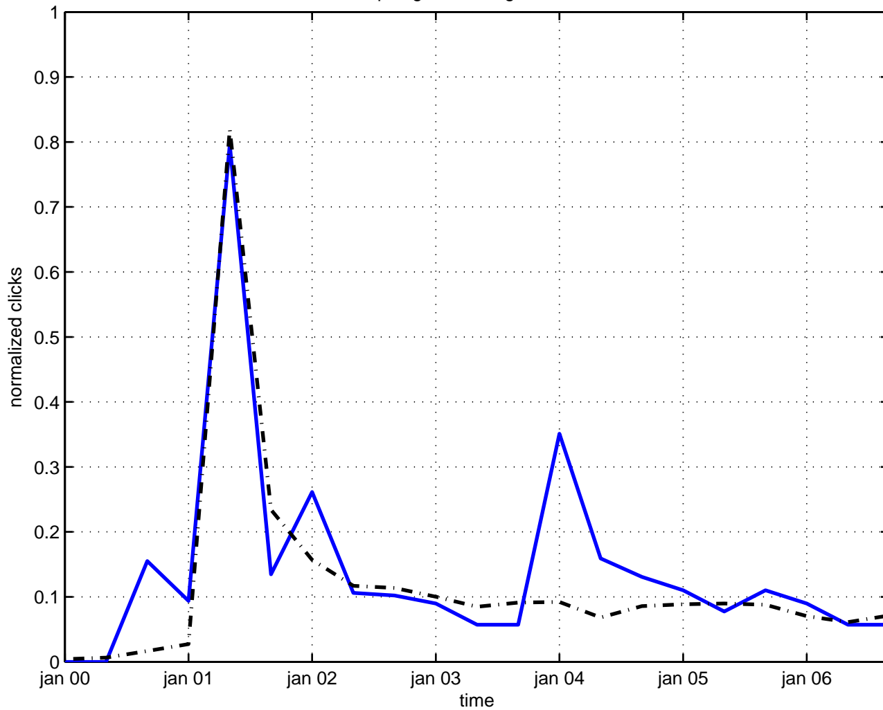
topological mass generation
