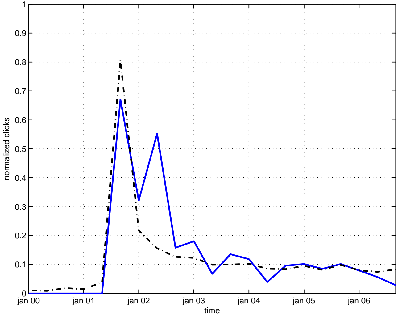
topological kink
