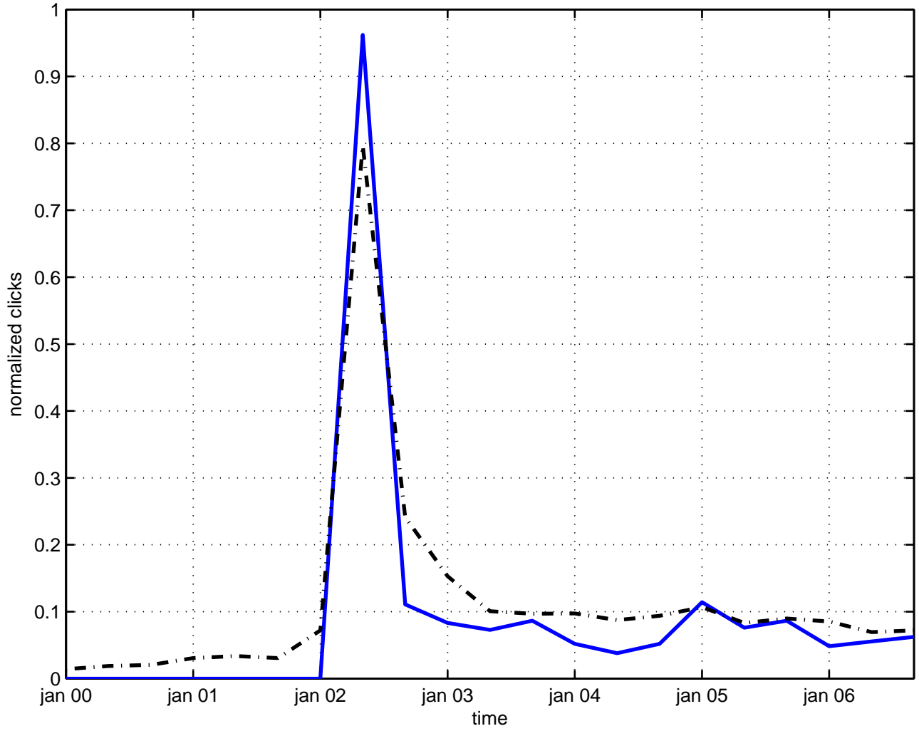
topological interaction
