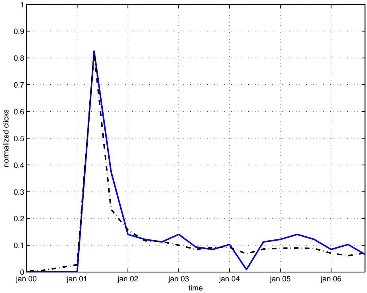
topological fusion
