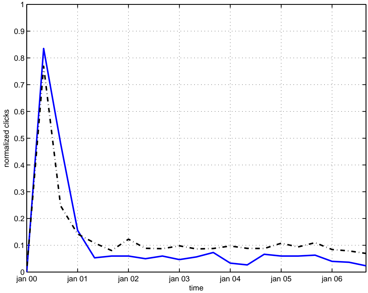
topological flux
