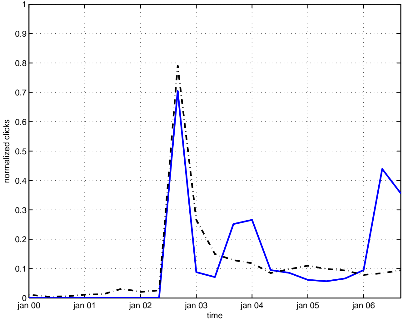
topological fluctuation
