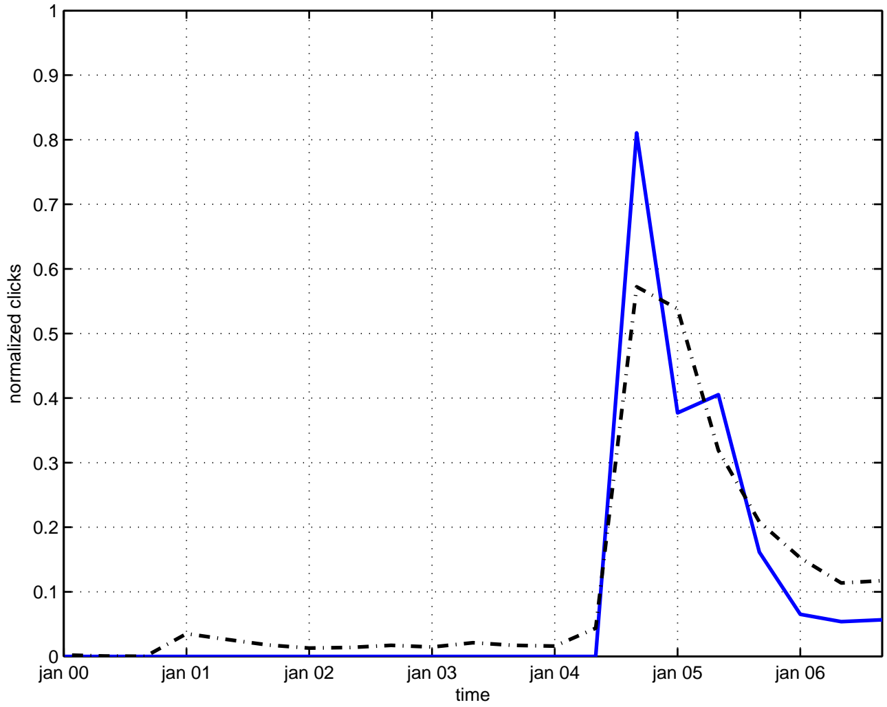
topological f-theory
