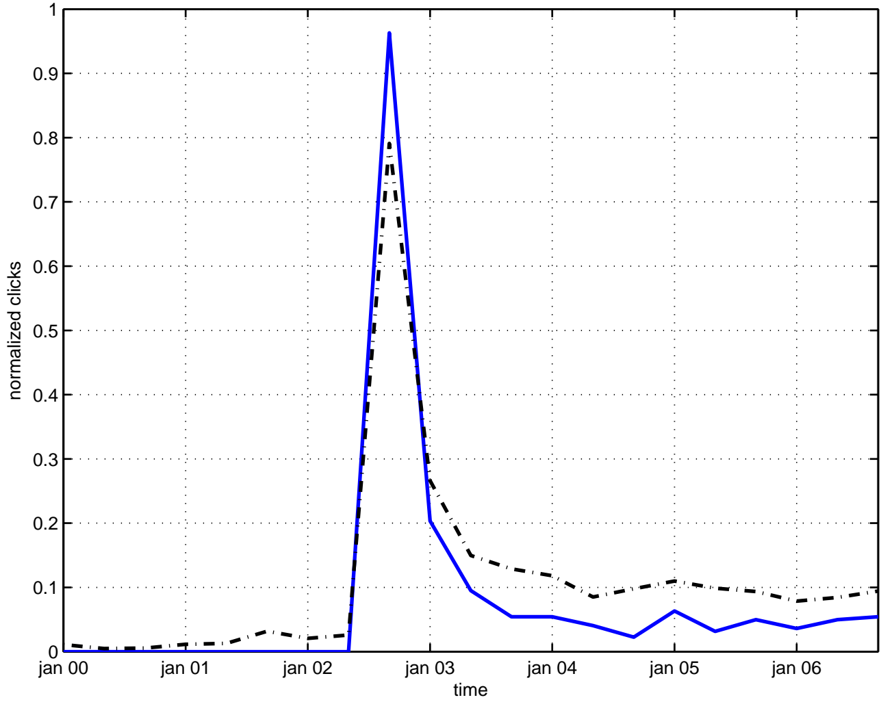
topological energy
