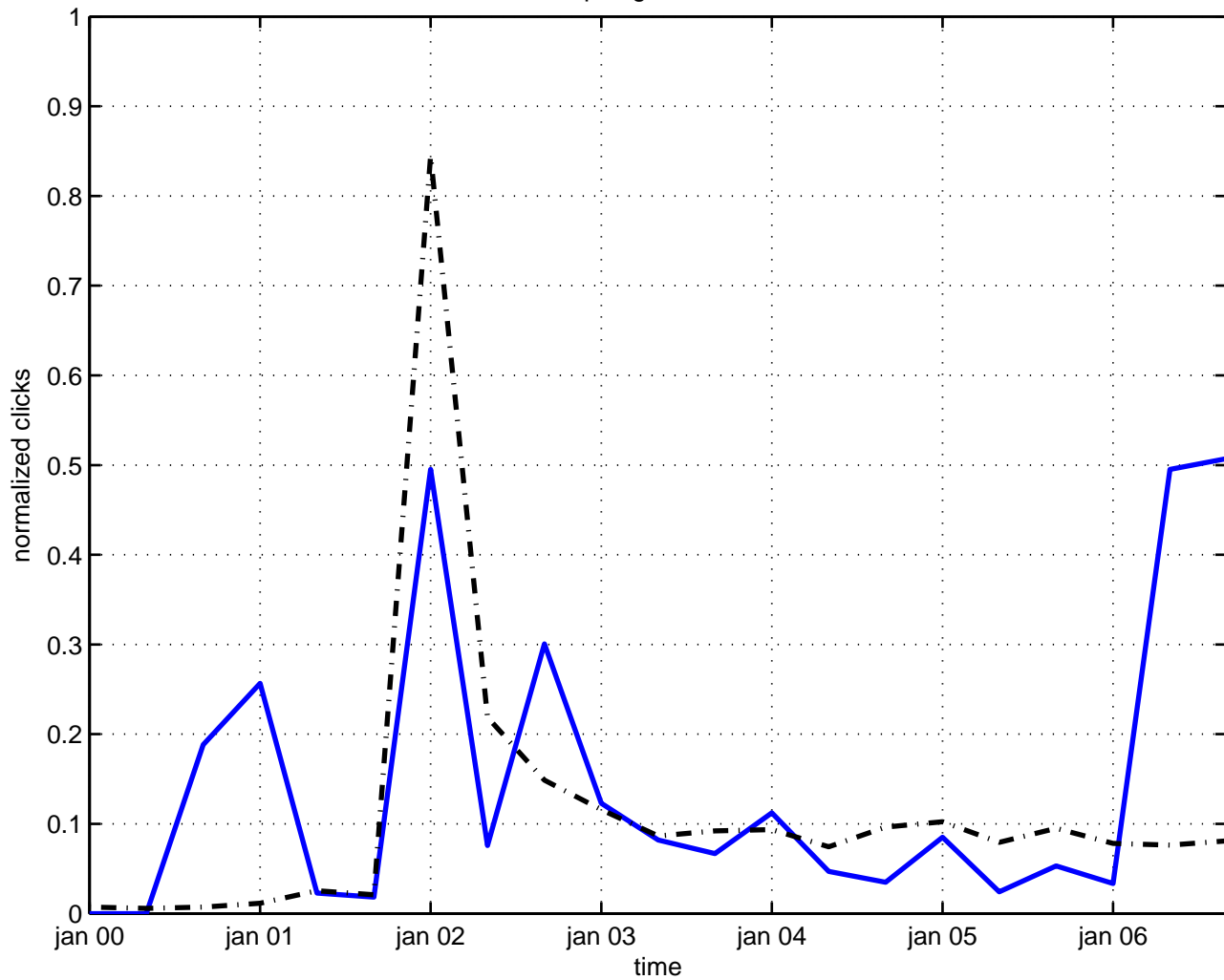
topological effect
