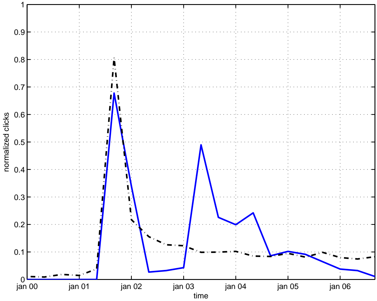
topological density
