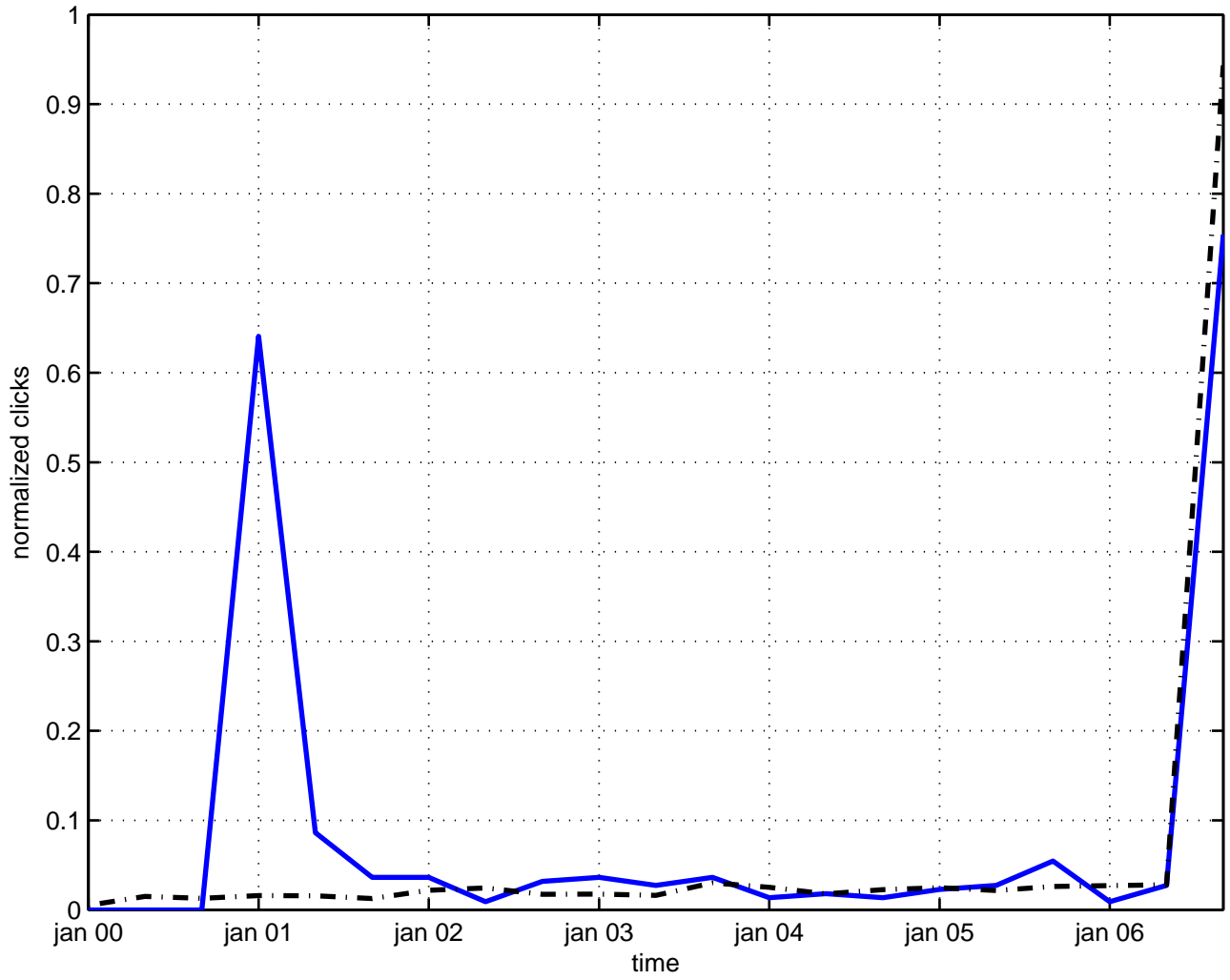
topological action
