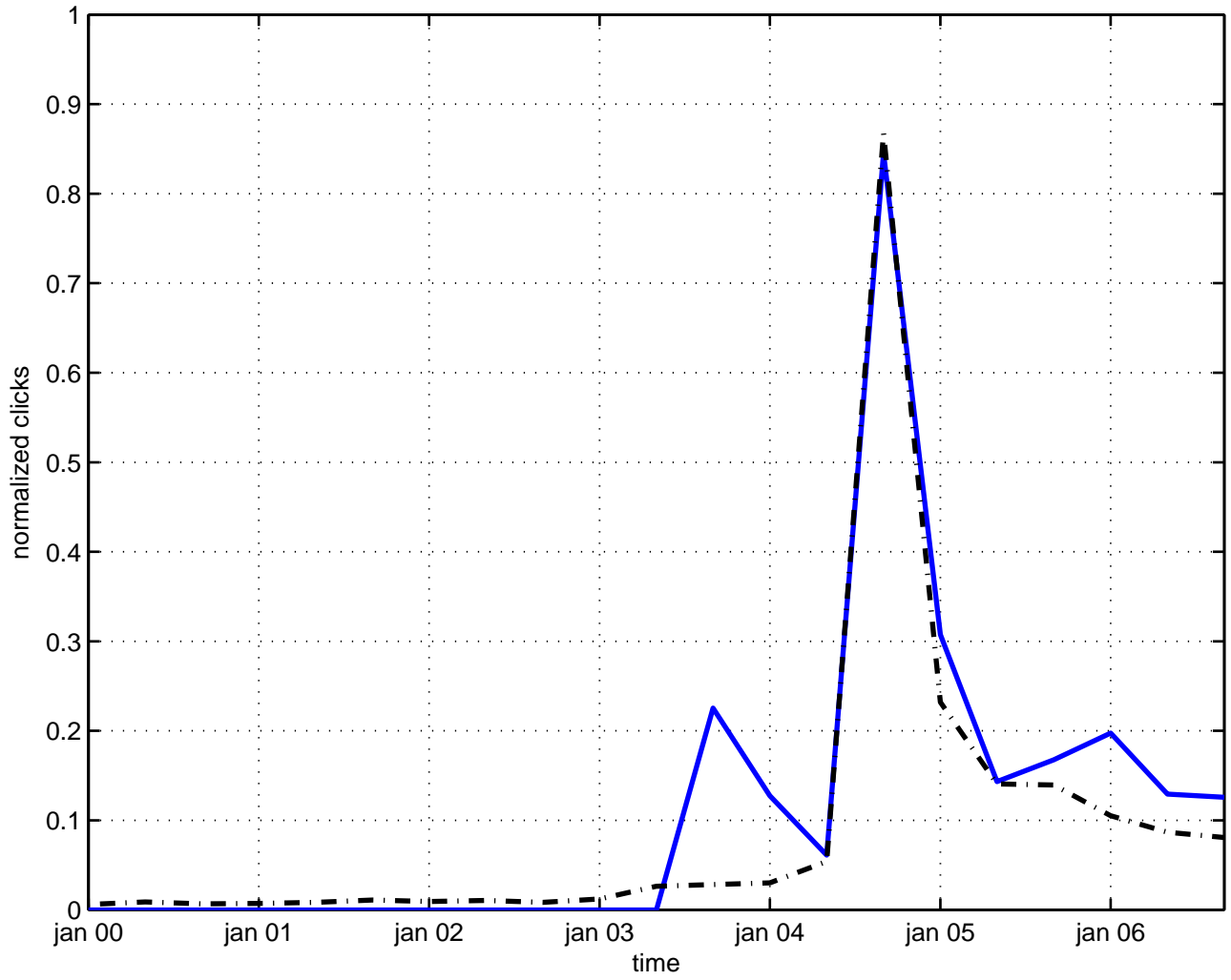
toda lattice field theory
