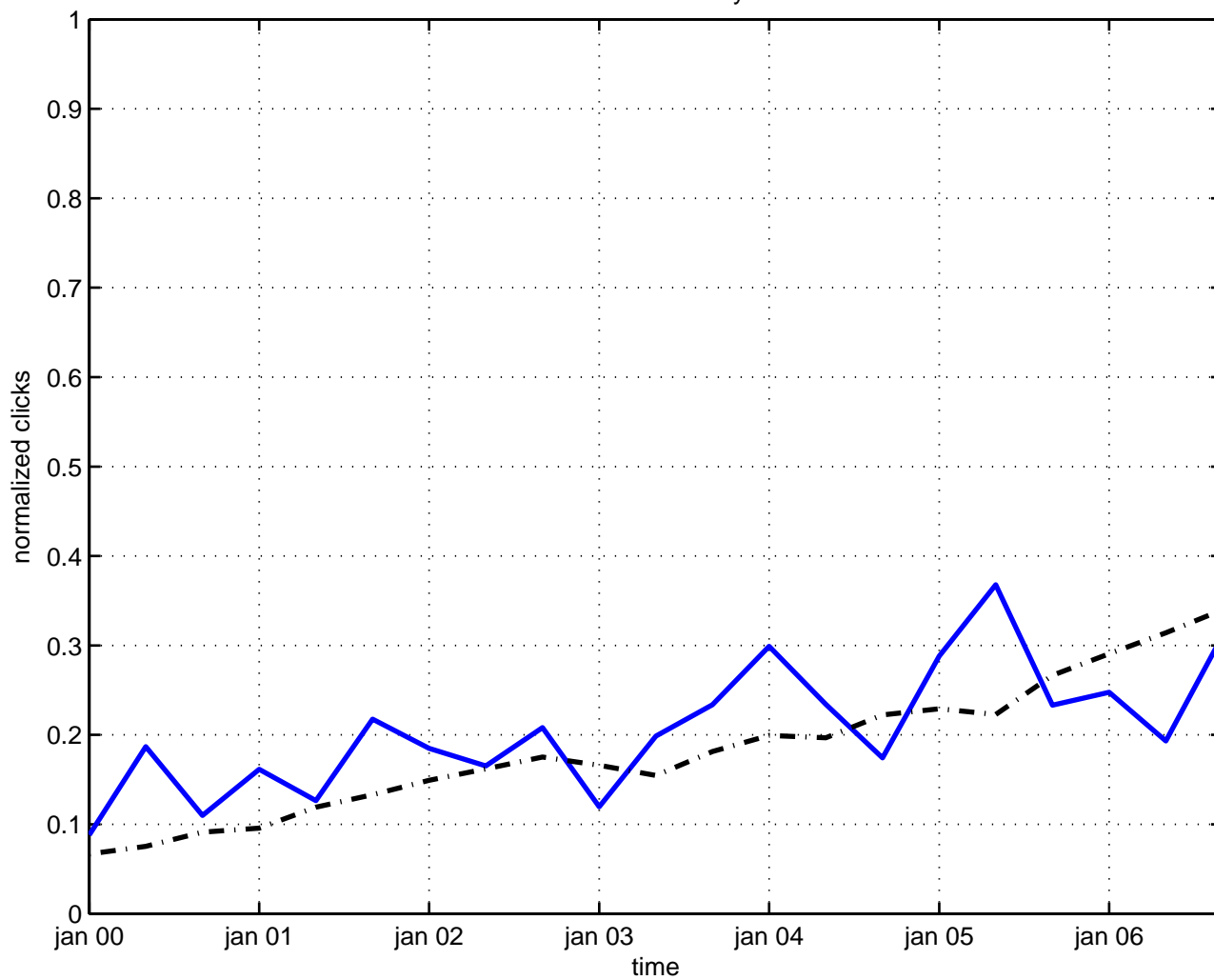
toda field theory
