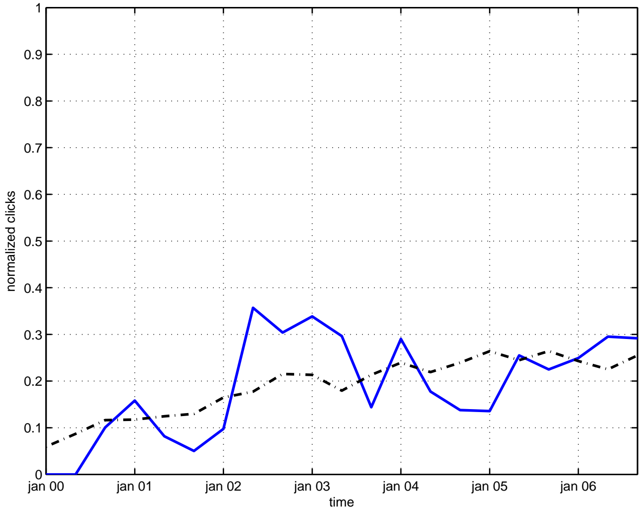
time reversal
