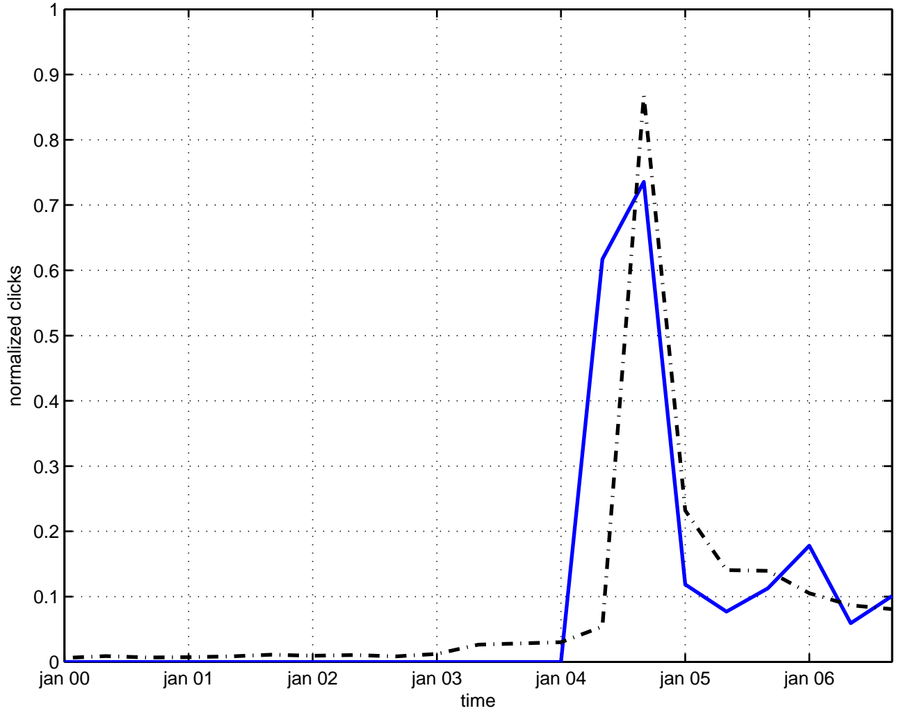
time reversal violation
