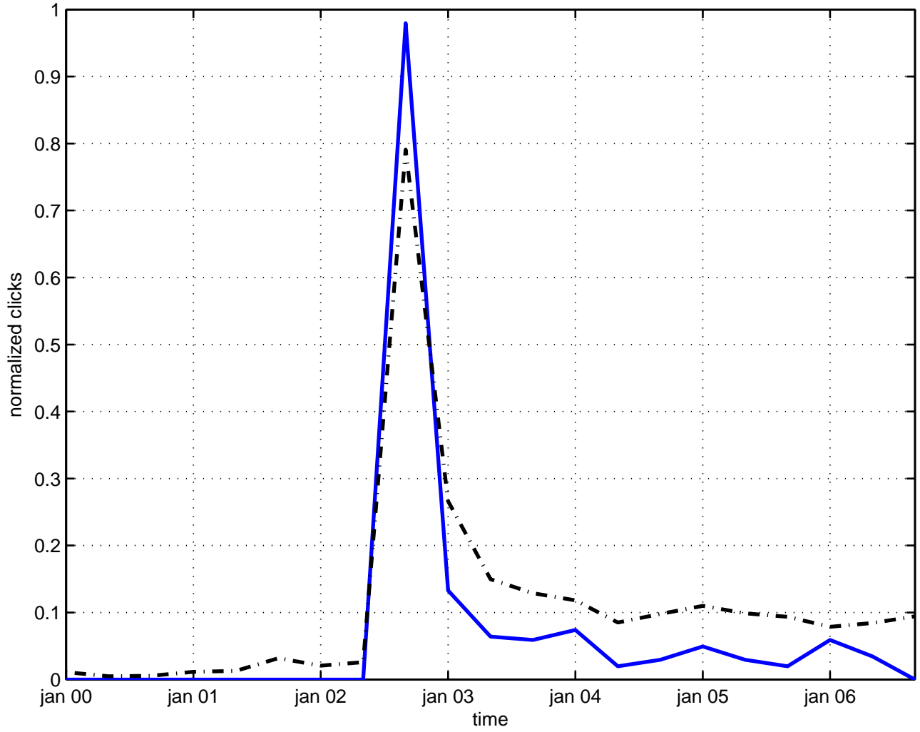
time dependence tachyon
