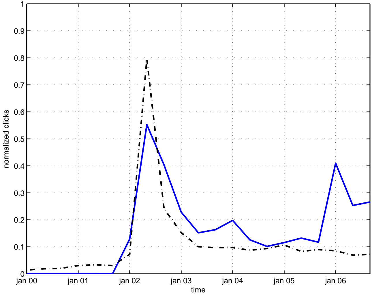
time dependence fundamental constant
