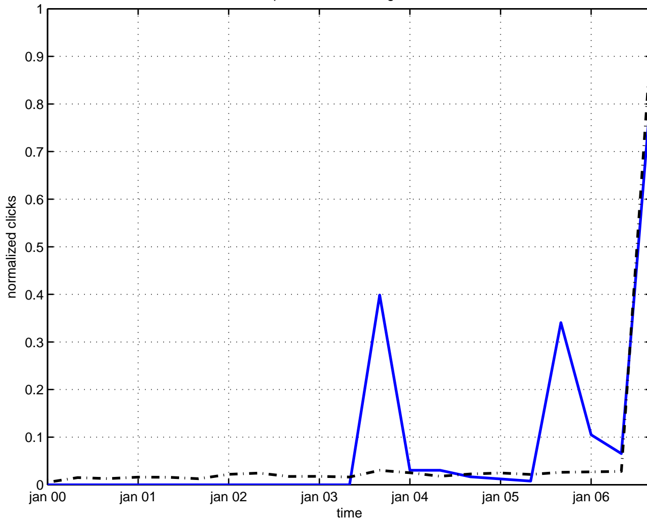
time dependence cosmological constant
