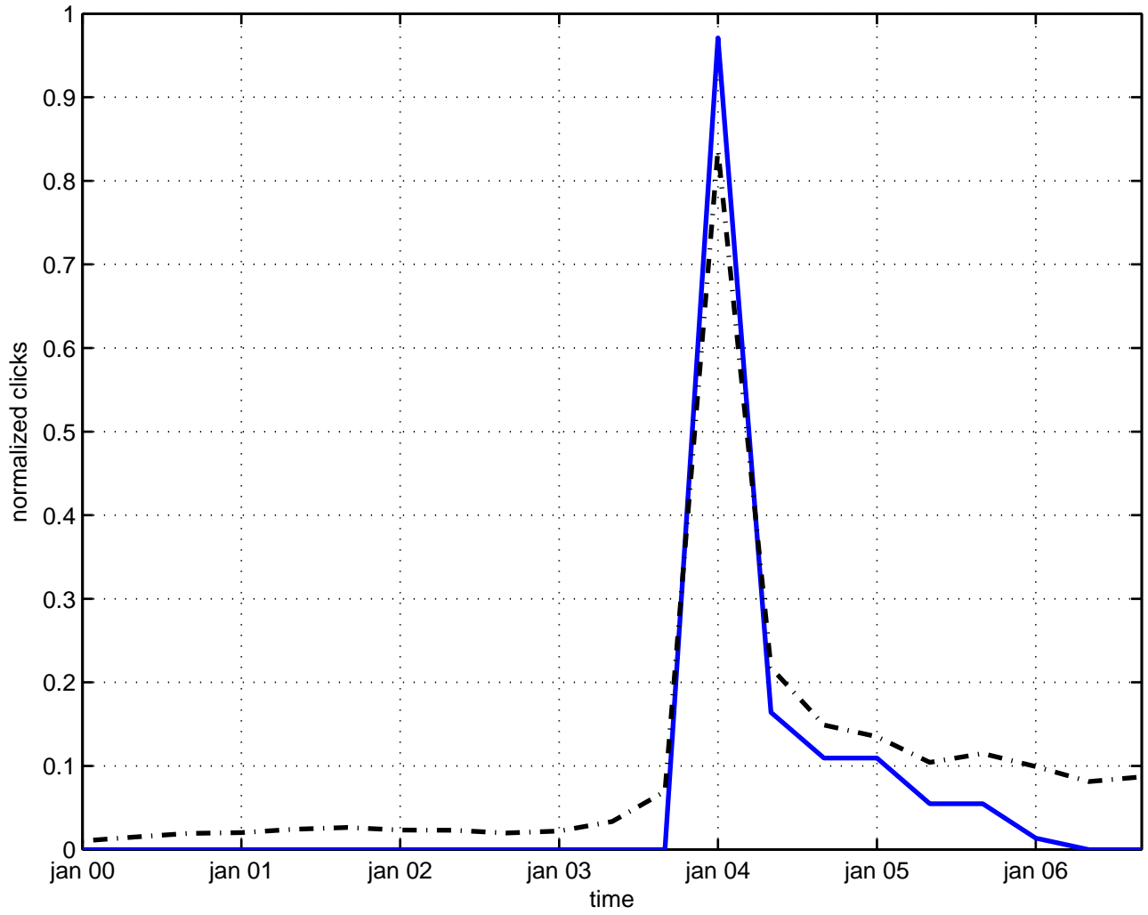
time delay graviton
