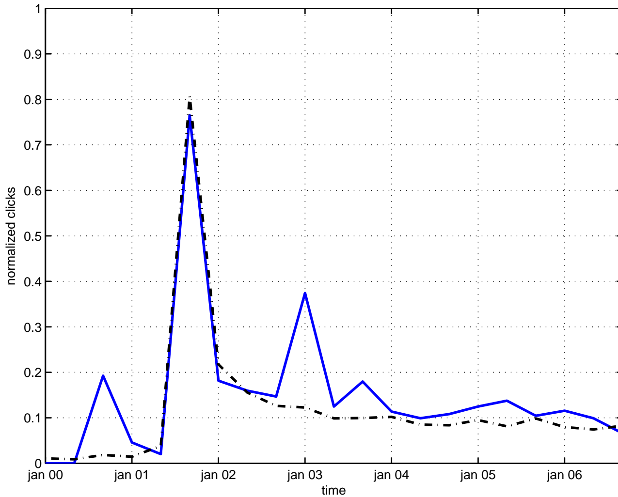
theta function
