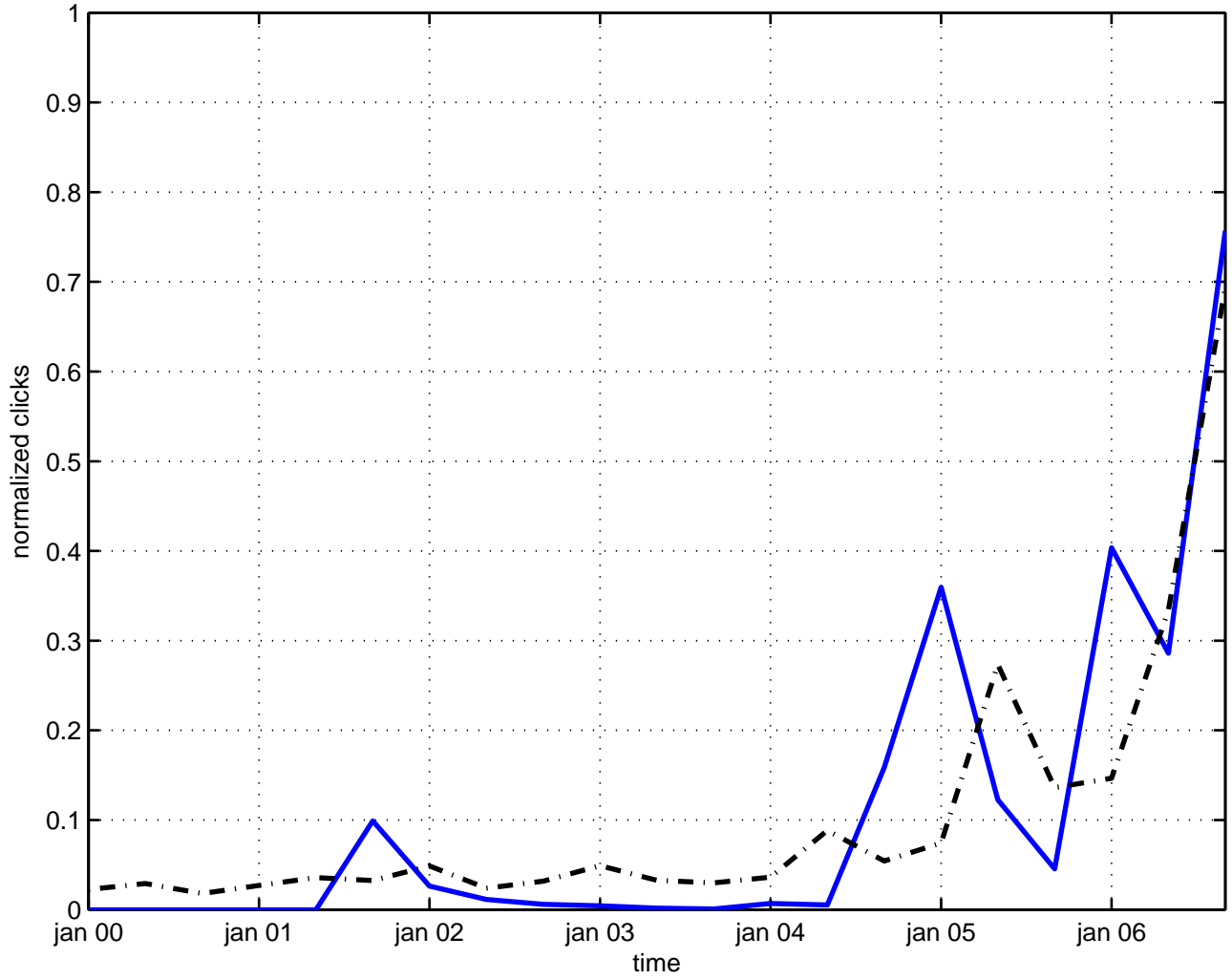
thermodynamics black hole
