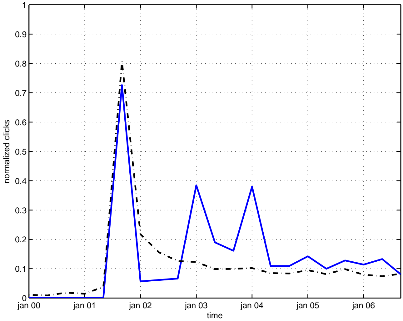
tensor torsion
