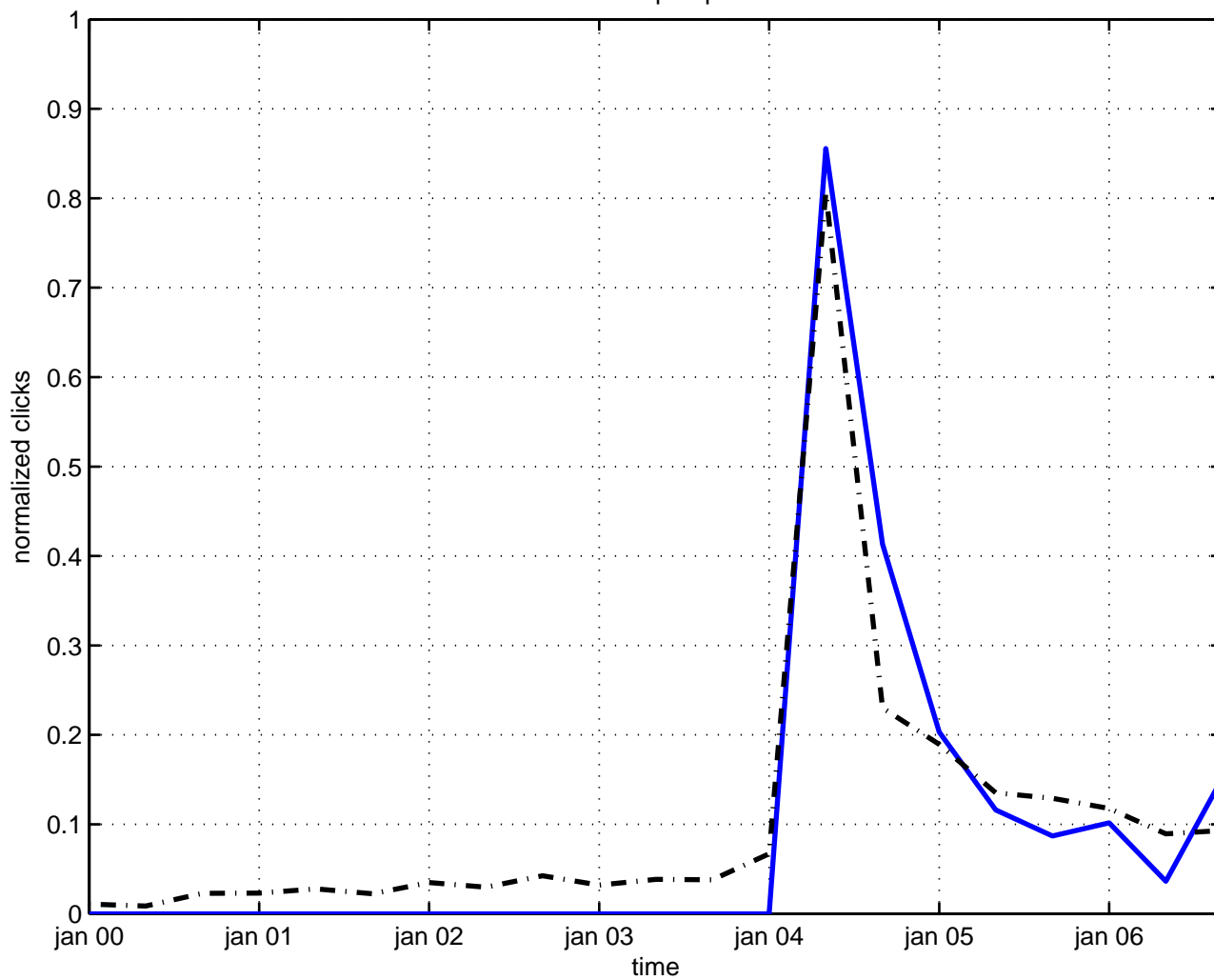
tensor superspace
