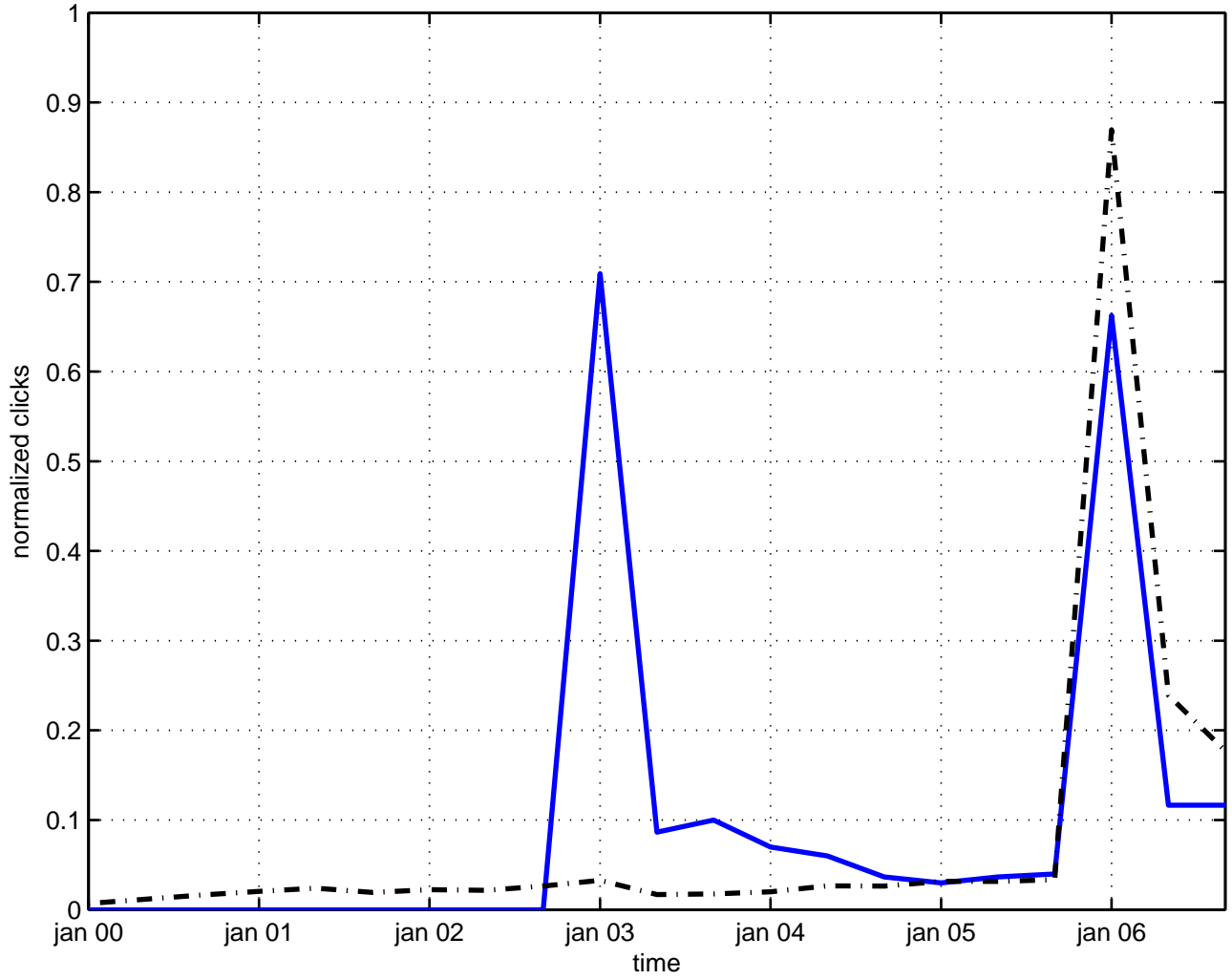
tensor space-time
