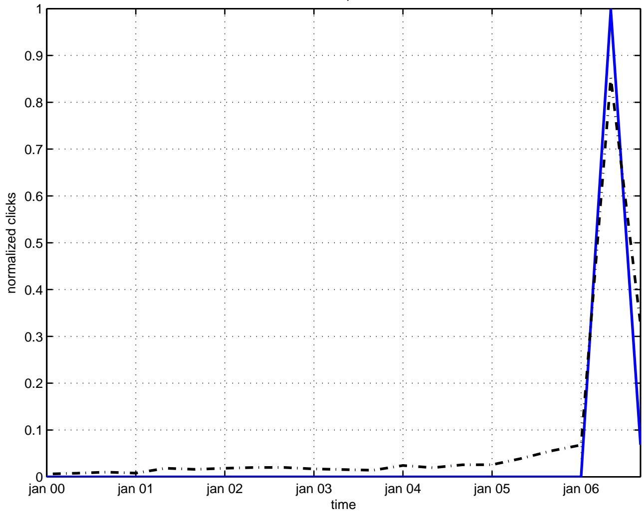
tensor operator
