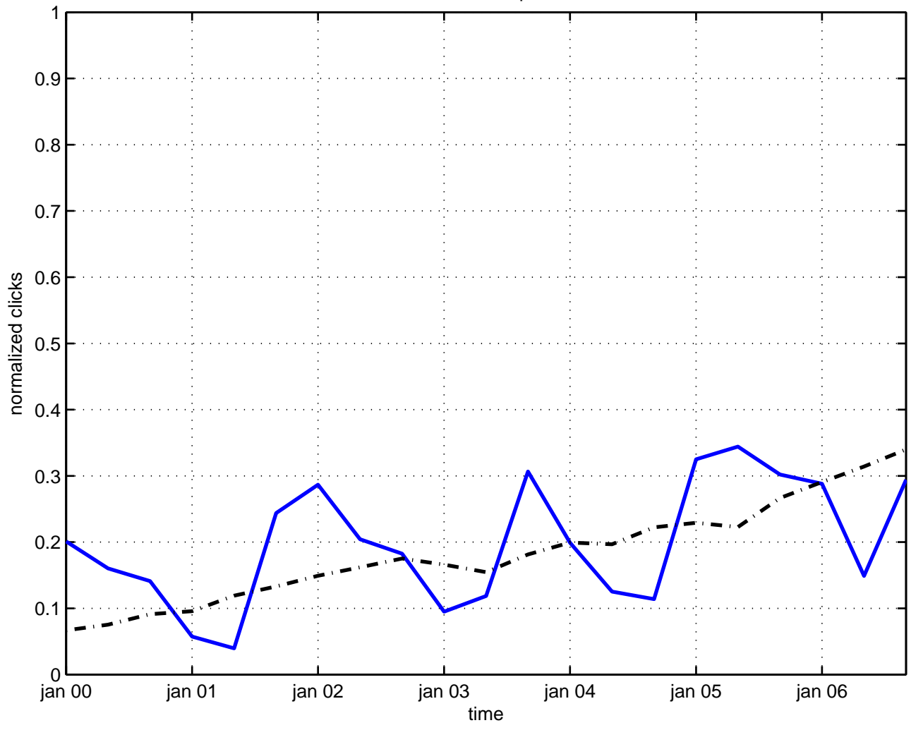
tensor multiplet
