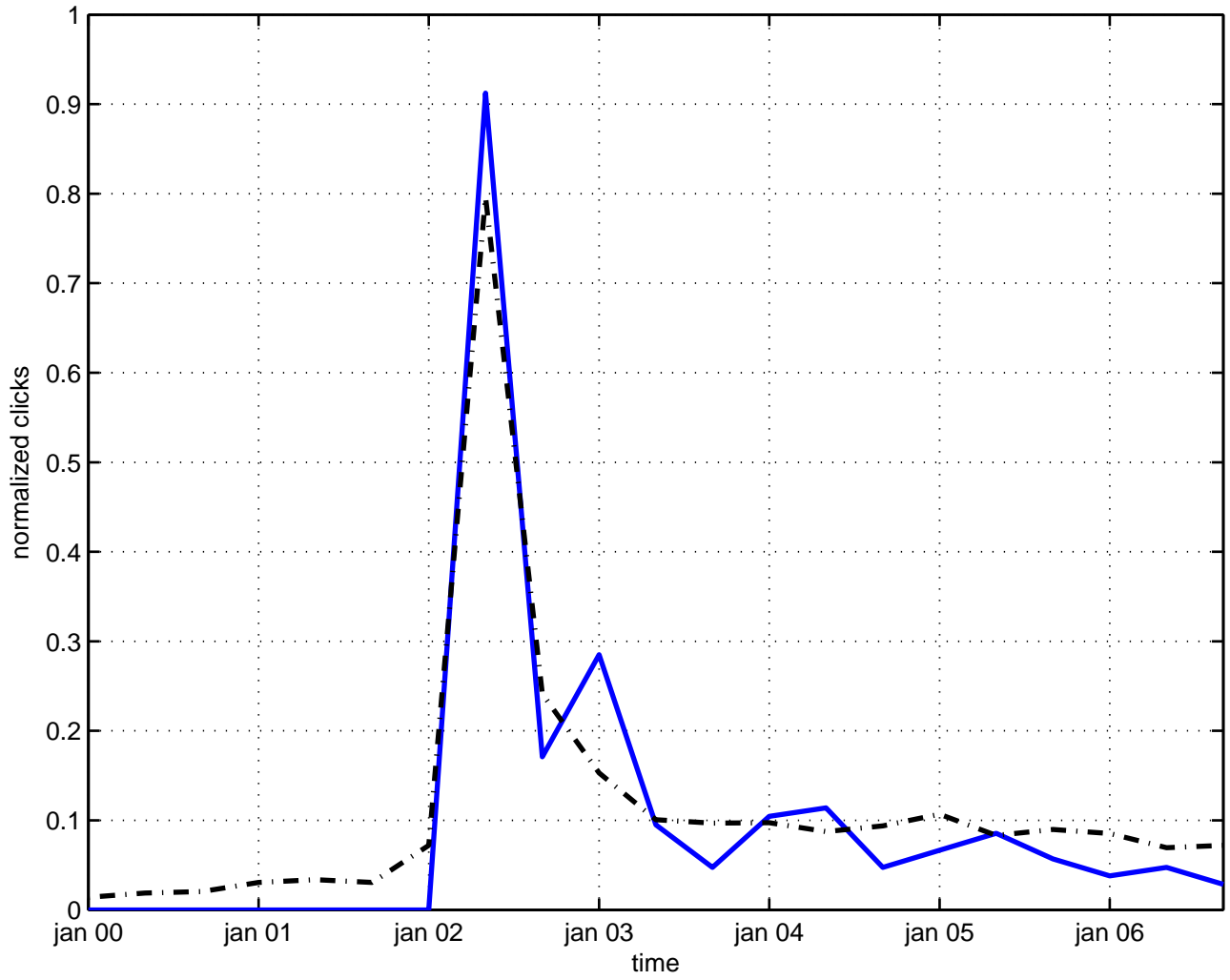
tensor model
