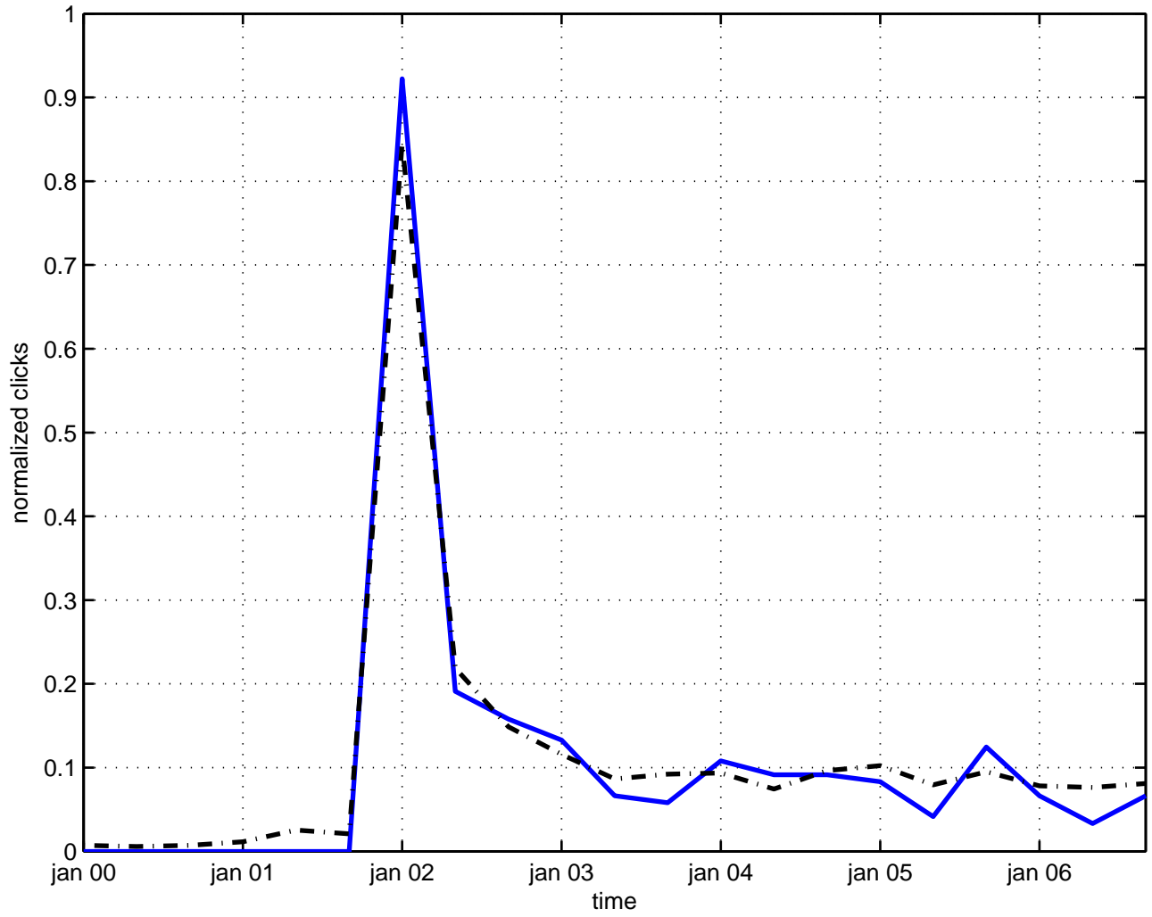
tensor matter
