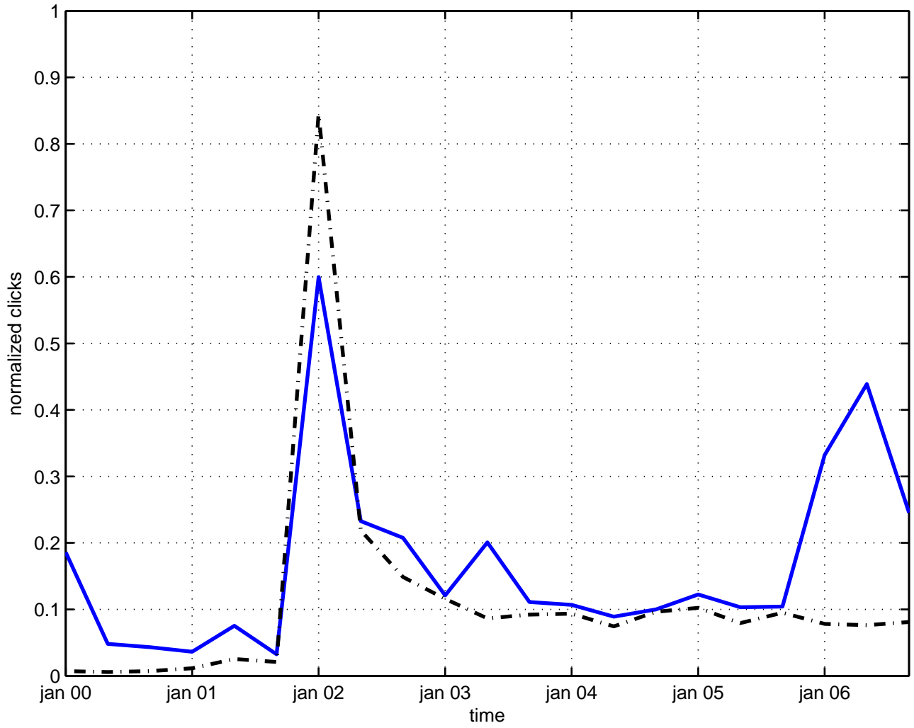
tensor fluctuation
