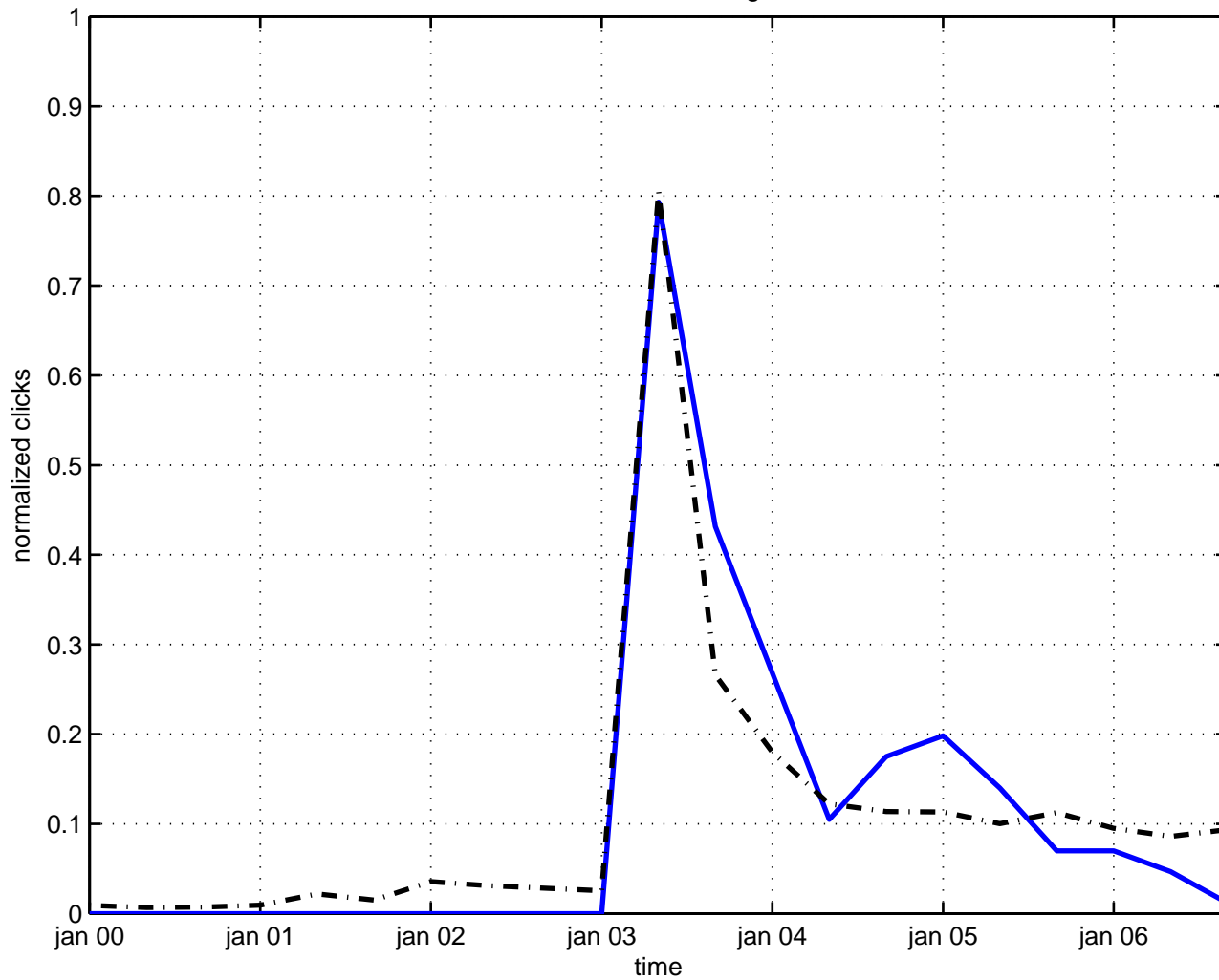
tensor embedding
