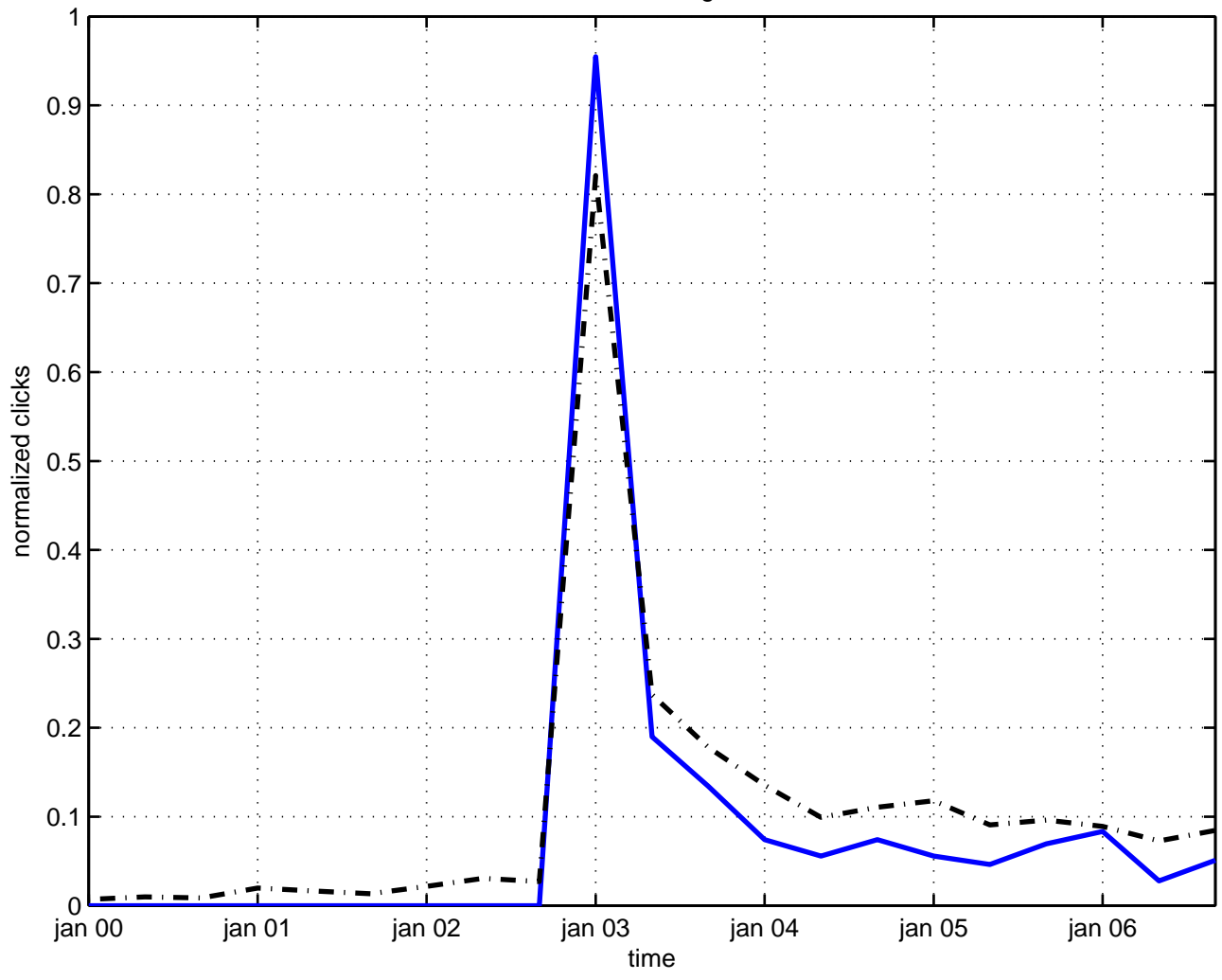
tensor charge
