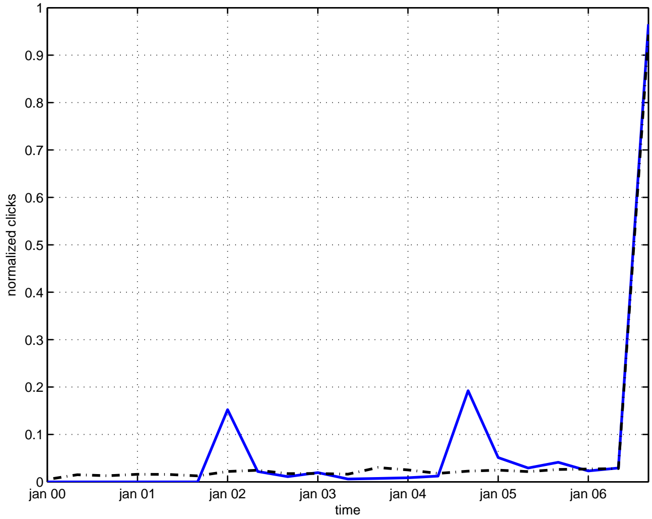
tensor algebra
