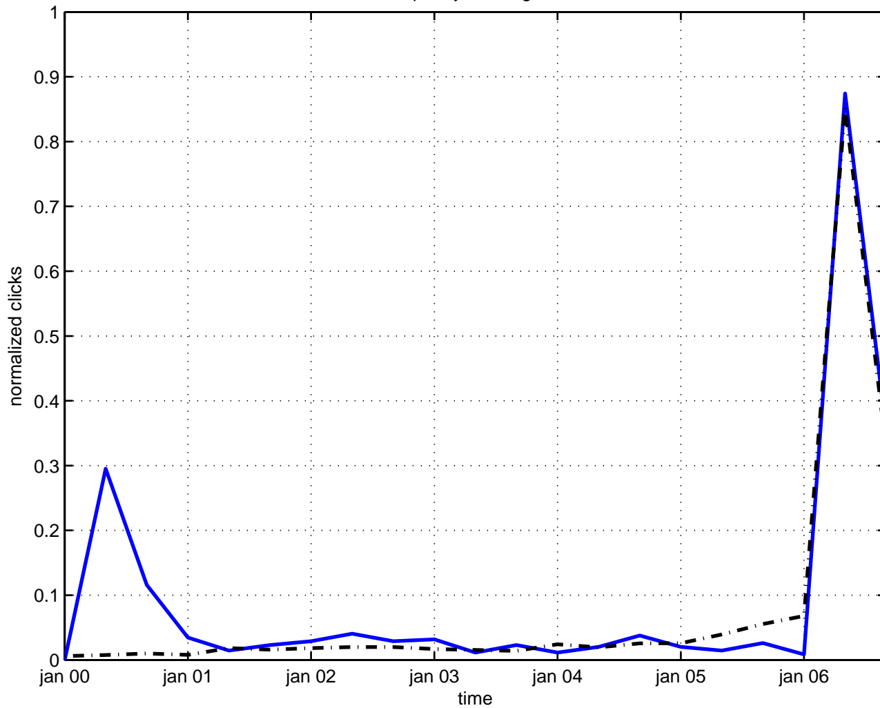
temperley–lieb algebra
