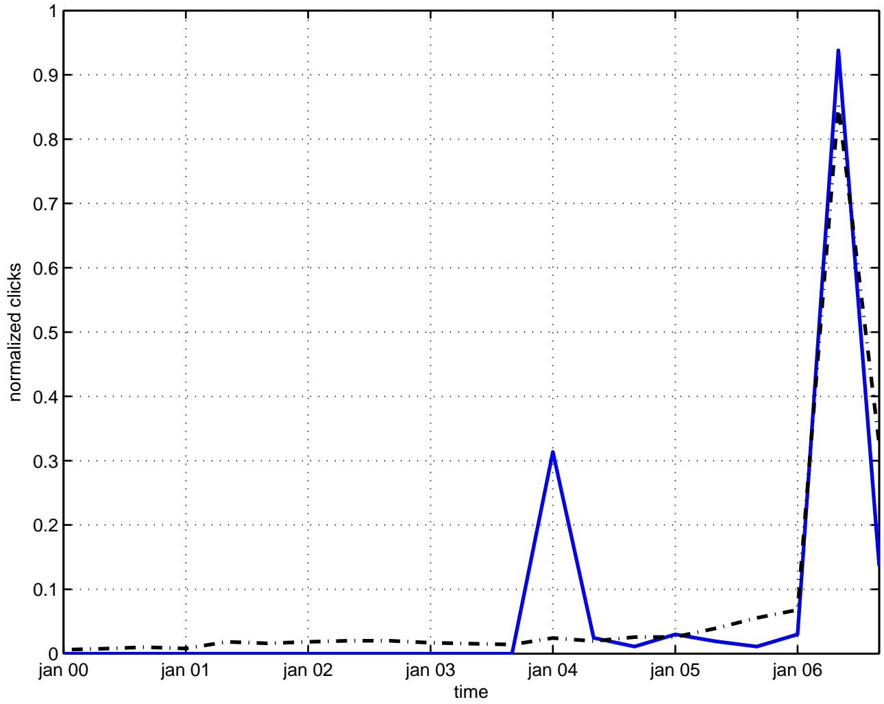
temperature radiation
