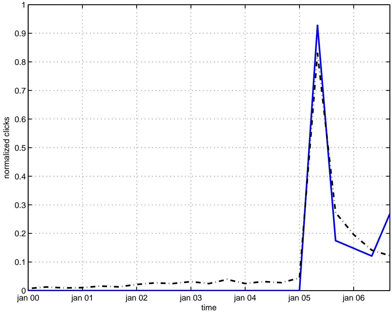
taylor expansion
