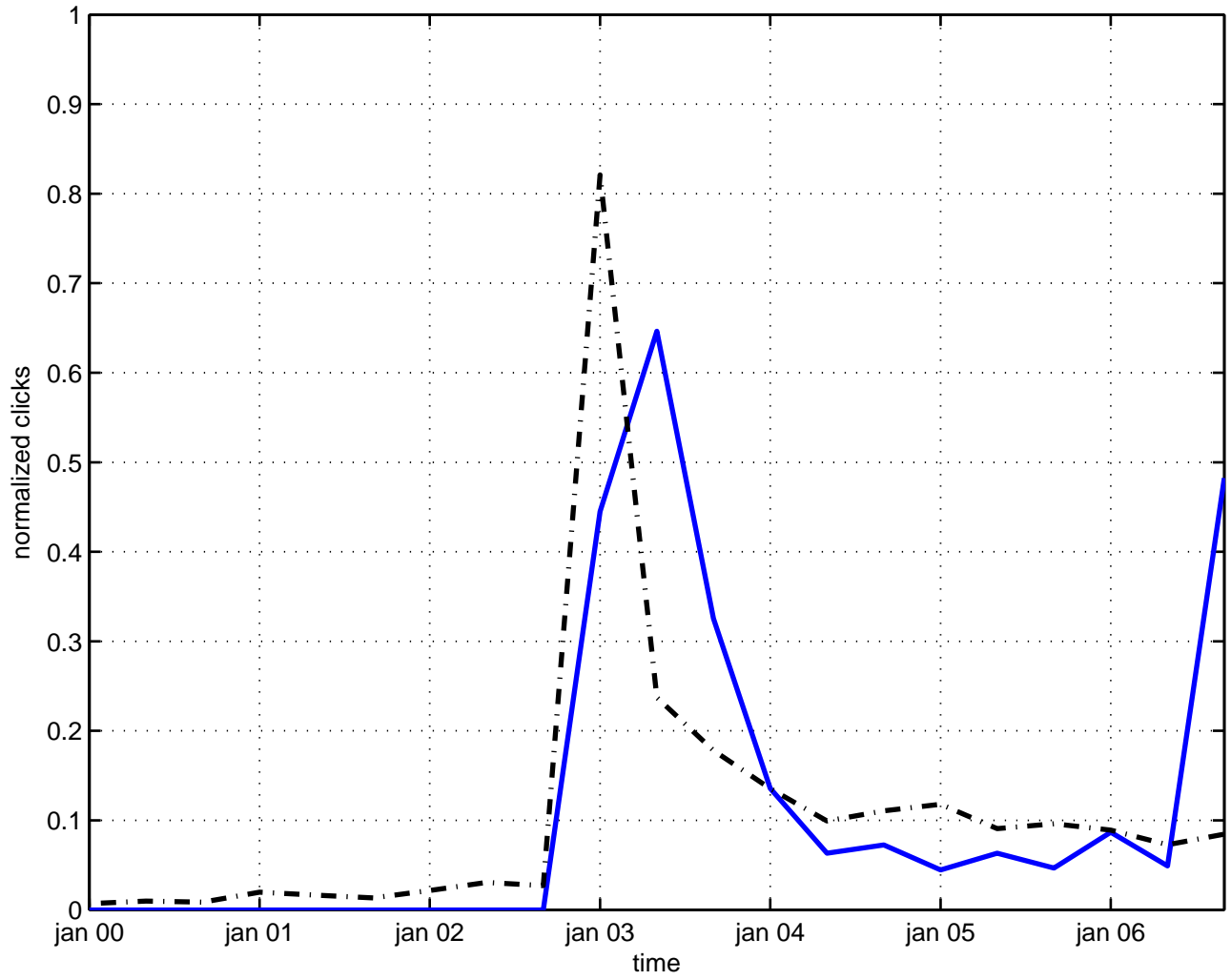
tadpole graviton
