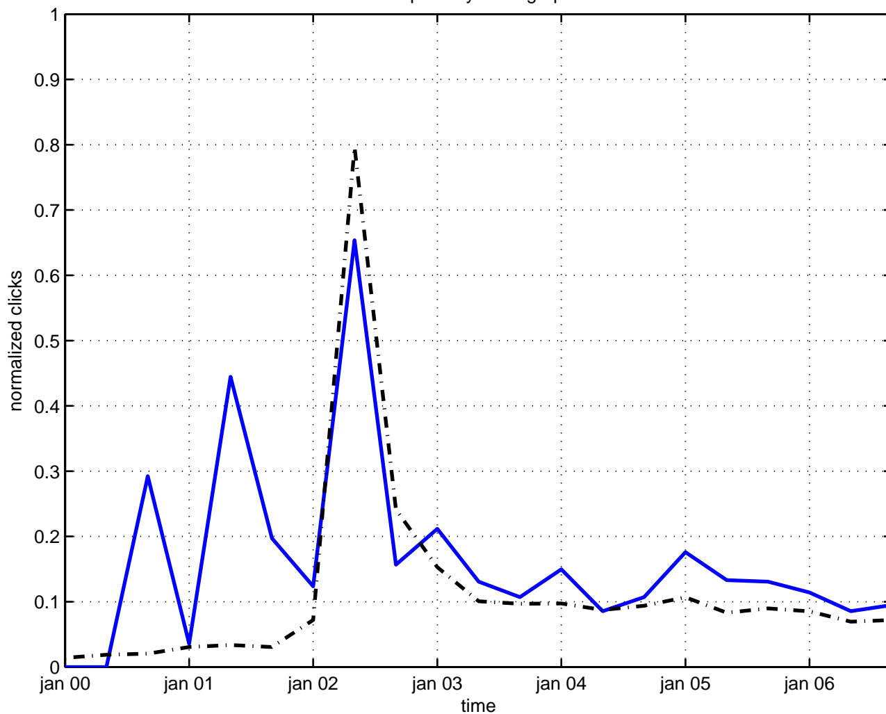
tadpole feynman graph
