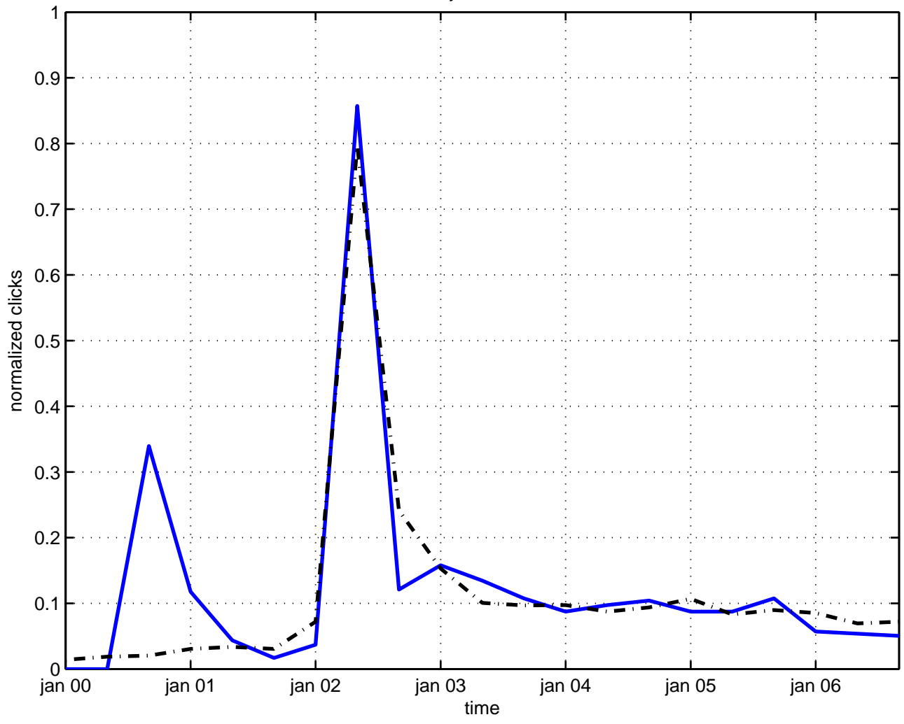
tachyon neutrino
