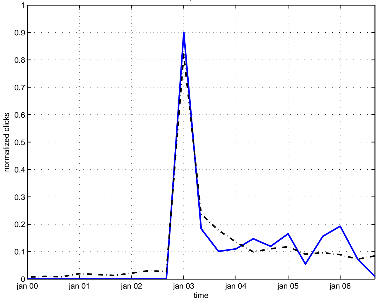
tachyon dilaton
