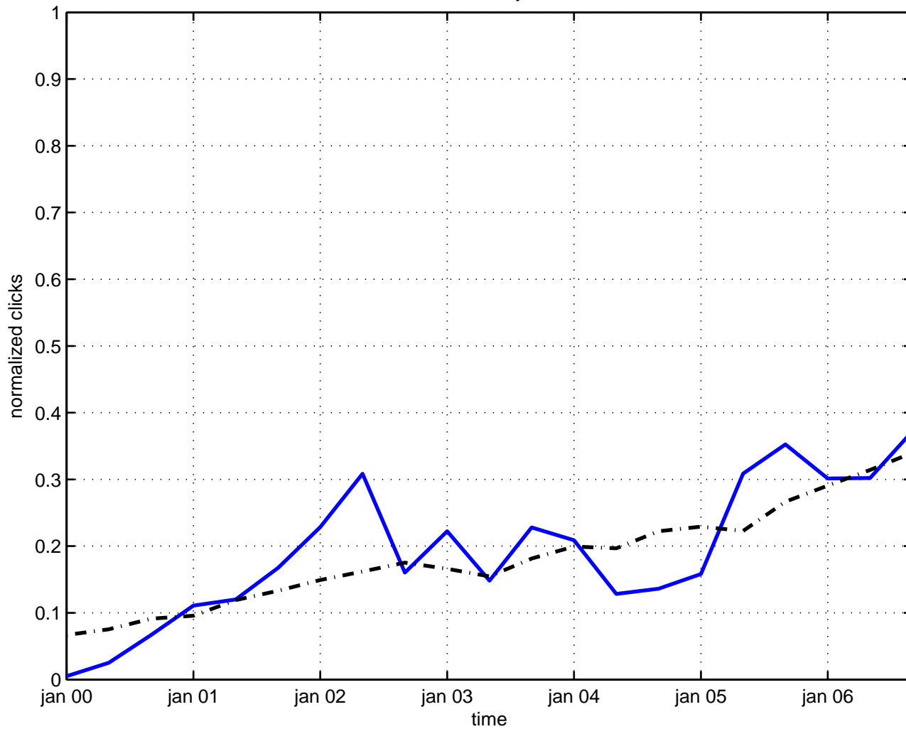
t-duality
